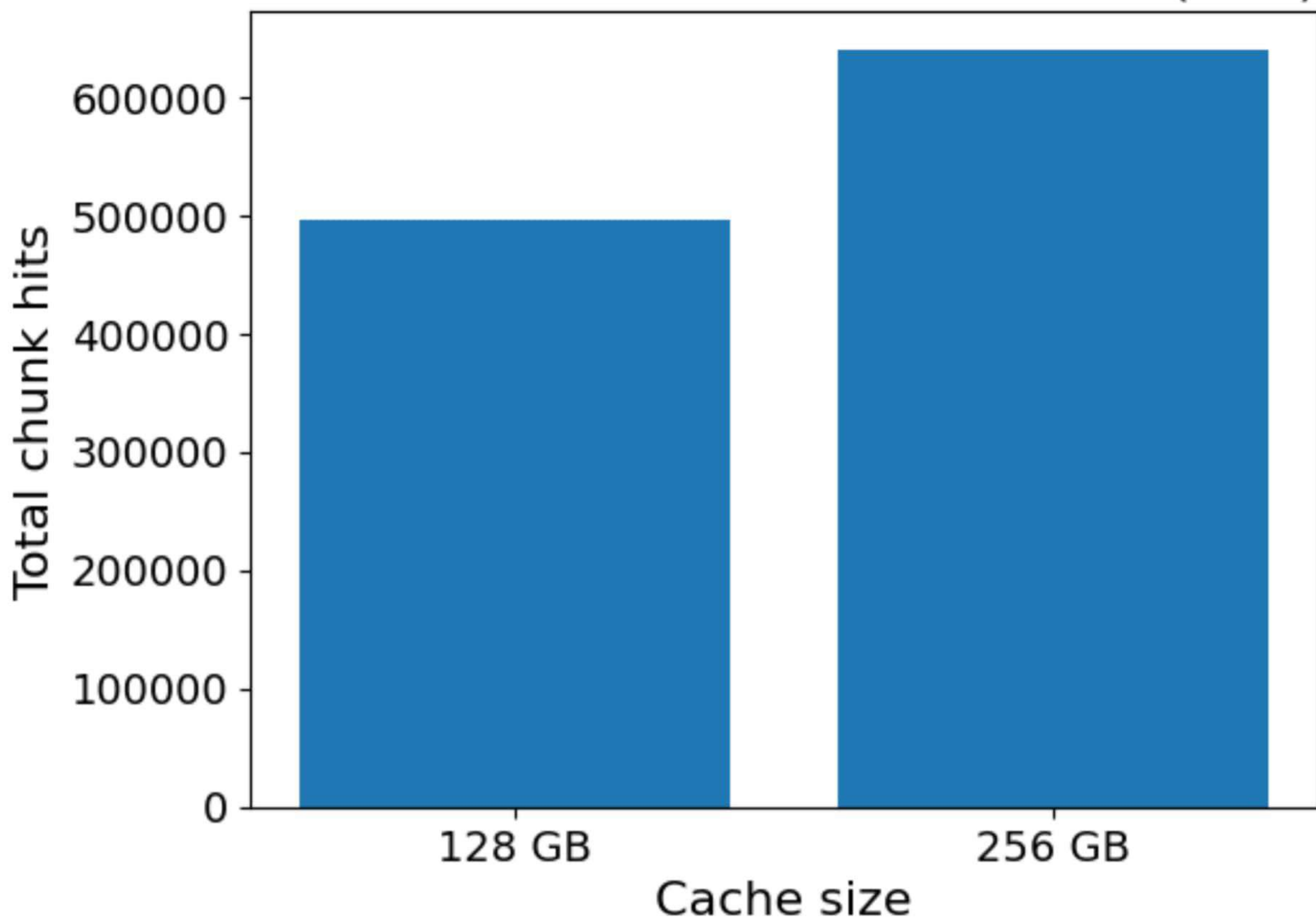
Effect of cache size on chunk hits (LRU)
